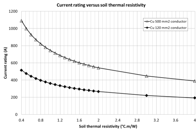
Fig. 8, Current rating vs native soil thermal resistivity.
