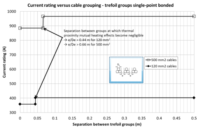
Fig. 5, Current rating vs separation between trefoil groups.
