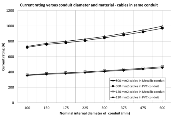
Fig. 10, Current rating vs conduit diameter.
