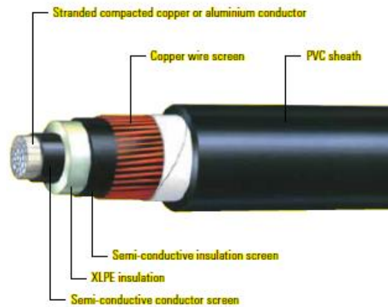
Fig. 13, Cross-sectional view of 11 kV cable modelled.
