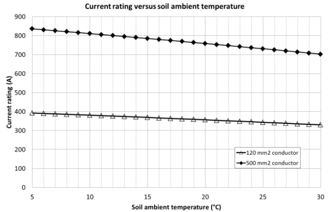
Fig. 11, Current rating vs soil ambient temperature.
