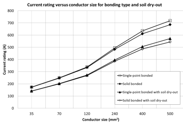
Fig. 6, Current rating vs conductor size – cables direct buried.
