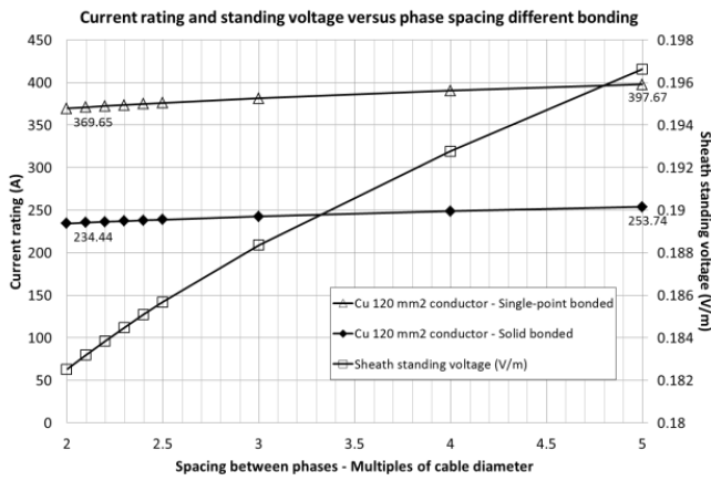
Fig. 9, Current rating and sheath standing voltage (single-point bonded cables) vs spacing between phases.
