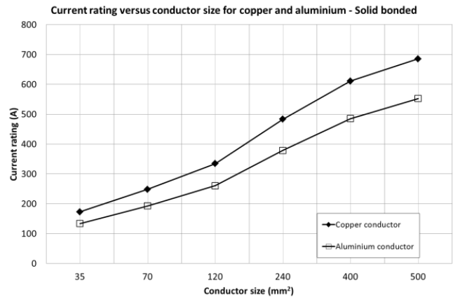
Fig. 7, Current rating vs conductor size for copper and aluminium conductors – cables direct buried.
