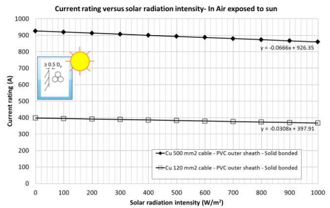
Fig. 3, Current rating of 120 mm 2 and 500 mm 2 cables exposed to varying solar radiation intensity.
