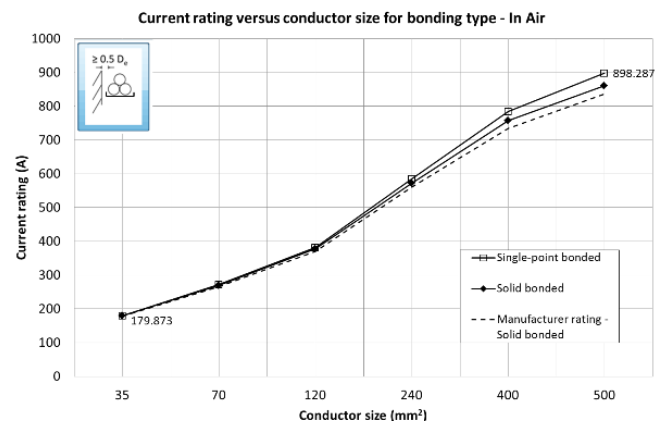
Fig. 1, Current rating vs conductor size – cables in air.
