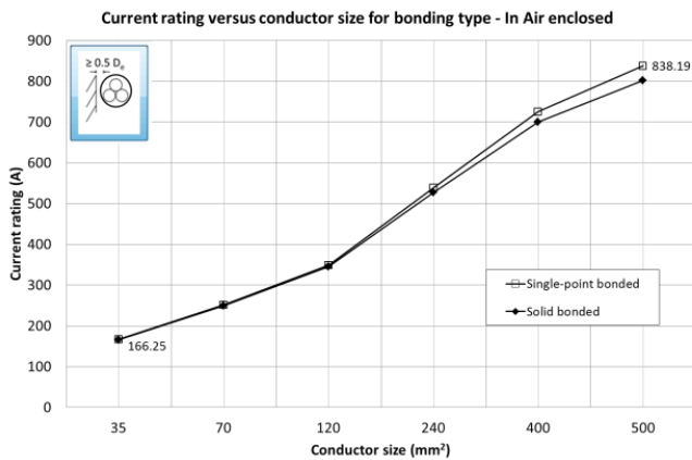
Fig. 2, Current rating vs conductor size for bonding type – cables in air enclosed in conduits.
