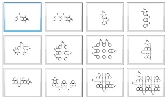
Fig. 4, Cables installed in groups – standardised arrangements as defined in IEC 60287-2-2 [3].
